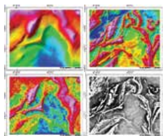
Gravity (top) and vertical gravity gradient (bottom)
